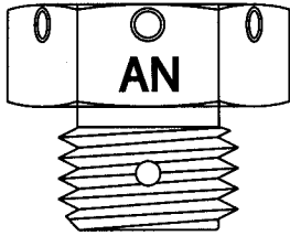
AN814, Bleeder Plug Add an "L" at the end for lockwire holes
