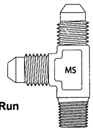
MS20825 and MS20826, Adapter Tees
