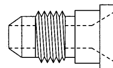
NAS1564, Female 37 Degree to Male 37 Degree
